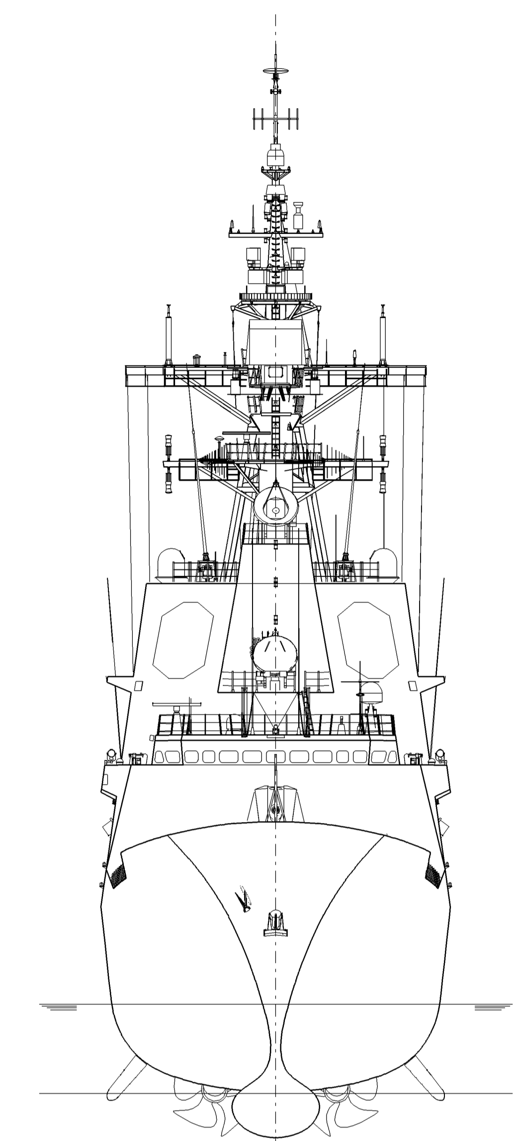
FORWARD VIEW
