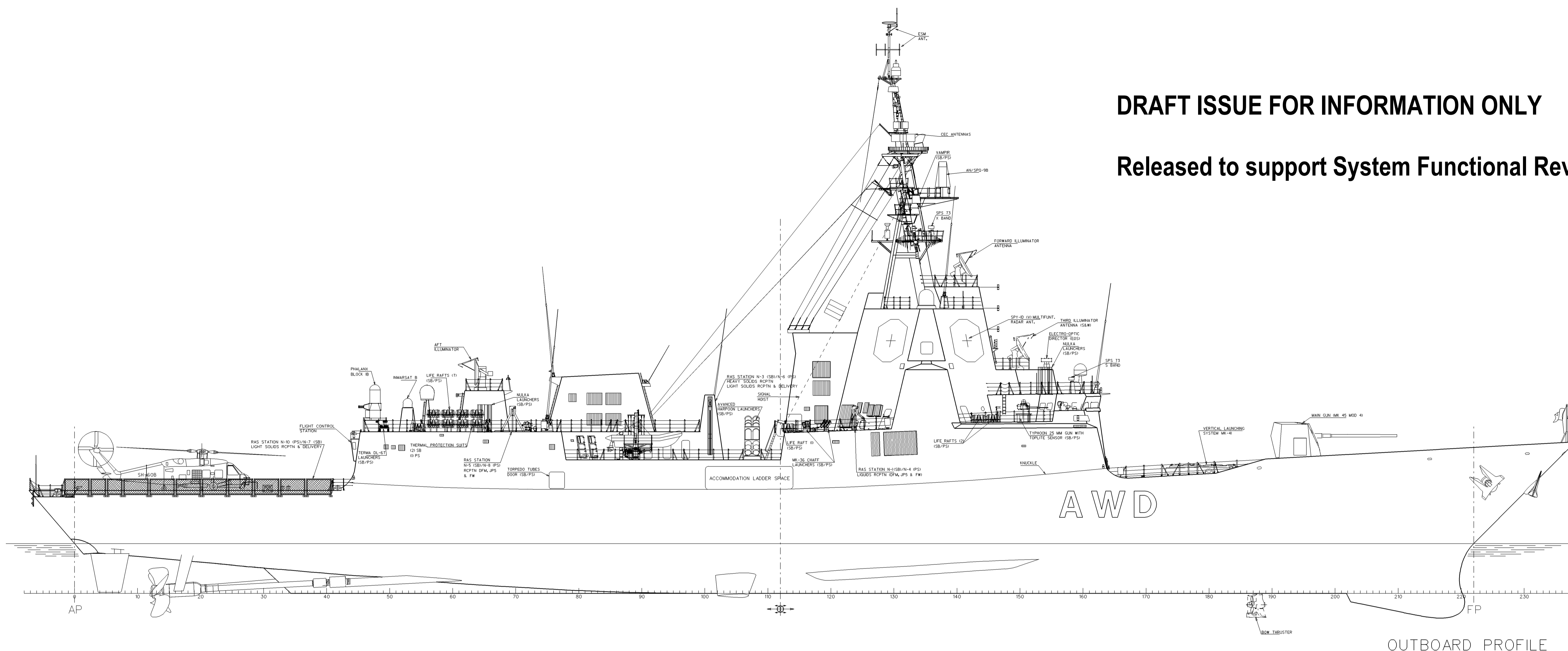
OUTBOARD PROFILE
